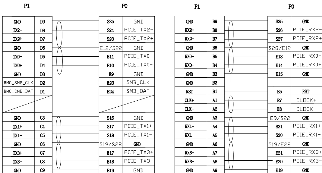
PIN ASSIGNMENT
