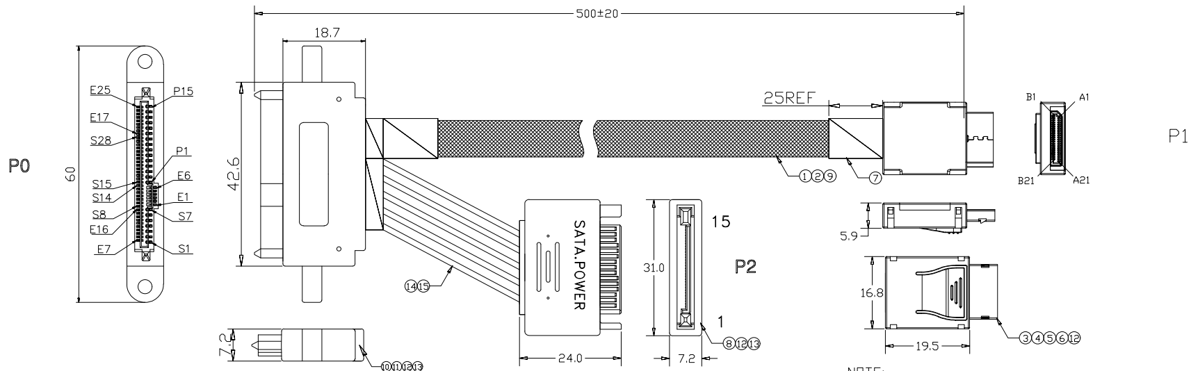
PIN ASSIGNMENT
