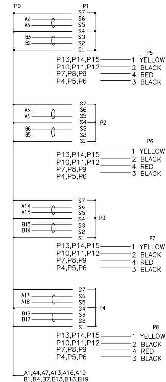
PIN ASSIGNMENT:
